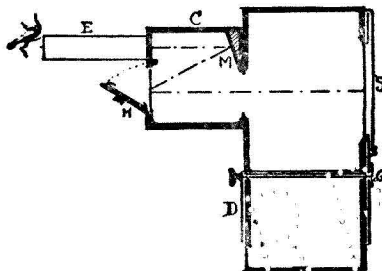
Vertical Section through light openings.
